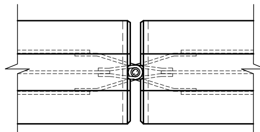
PLAN VIEW OF CONNECTION DETAIL
