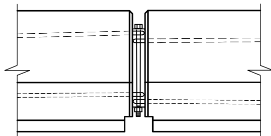
ELEVATION OF CONNECTION DETAIL
