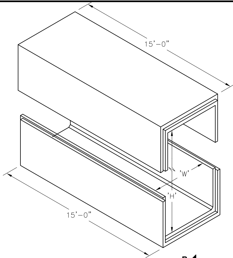
Box Culvert Type-II Top
