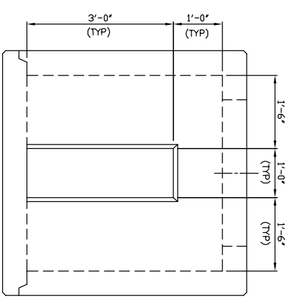
WALL #2 ELEVATION
