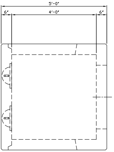
WALL #1 ELEVATION
