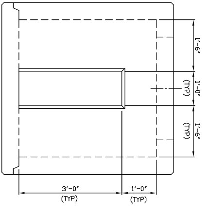
WALL #4 ELEVATION
