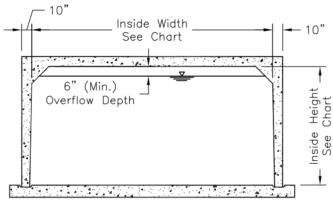
Section View
