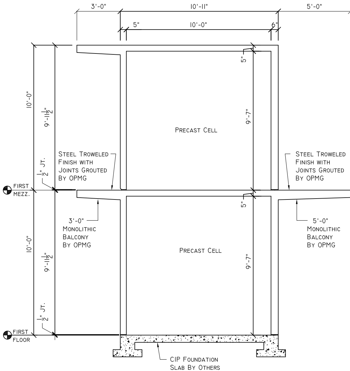
TYP. CELL CROSS SECTION 70 SQ. FT. PER CELL
