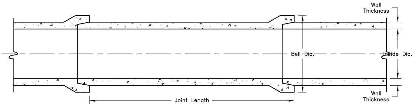
Assembled Cross Section
